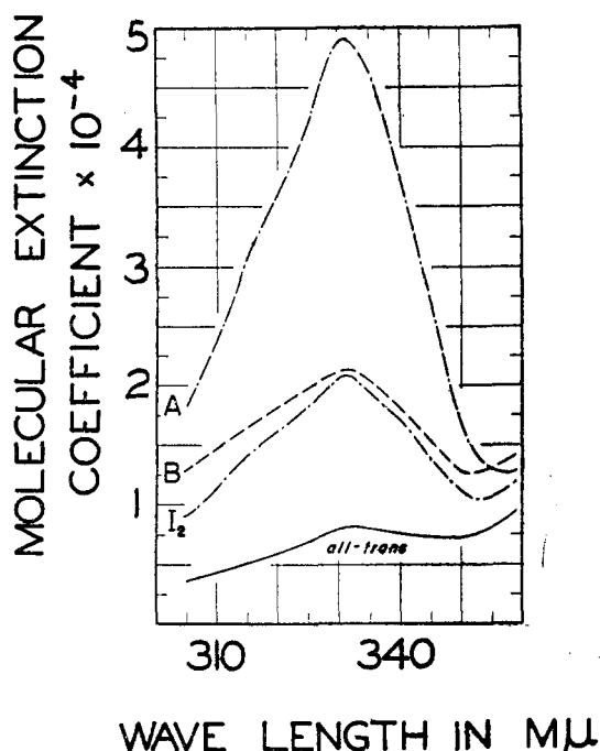
FIG. 28. Molecular extinction curves of some members of the stereoisomeric lutein set in the cis -peak region in hexane. I_2 indicates the equilibrium mixture obtained upon iodine catalysis at room temperature in light. (From J. Am. Chem. Soc. 66 , 140 (1944))
