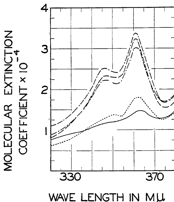
FIG. 14. Influence of illumination on the development of the cis -peak in an iodine-catalyzed solution of all- trans -lycopene in hexane: ····, molecular extinction curve after zero seconds; — — —, after 5 sec.; - - - -, after 30 sec.; — · — ·, after 15 min. illumination. The full line denotes the curve taken before the addition of iodine, without illumination. (From J. Am. Chem. Soc. 66 , 189 (1944))
