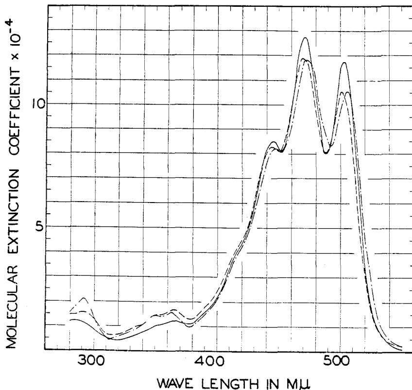
FIG. 30. Molecular extinction curves of natural methylbixin in benzene: —, fresh solution of natural methylbixin; ---, mixture of stereoisomers after refluxing in darkness for 45 min.; - · -, mixture of stereoisomers after iodine catalysis at room temperature in light. (From J. Am. Chem. Soc. 66 , 323 (1944))
