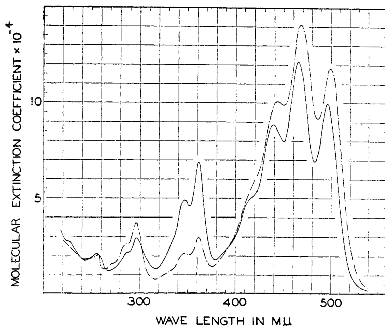
FIG. 19. Molecular extinction curves of neocyclope A in hexane: —, fresh solution of neocyclope A; ---, mixture of stereoisomers after iodine catalysis at room temperature in light. (From J. Am. Chem. Soc. 65 , 1944 (1943))
