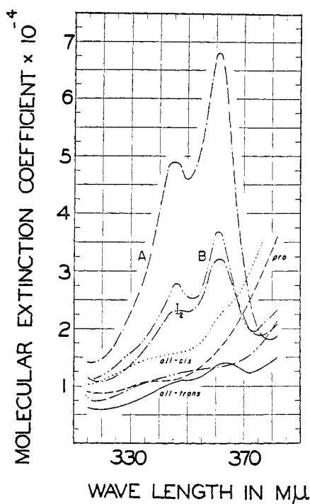
FIG. 20. Molecular extinction curves of some members of the stereoisomeric lycopene set in the cis -peak region in hexane: \cdots denotes an unnamed crystalline isomer; I_2 indicates the equilibrium mixture obtained upon iodine catalysis at room temperature in light. (From J. Am. Chem. Soc. 66 , 141 (1944))
