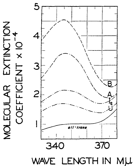
FIG. 24. Molecular extinction curves of some members of the stereoisomeric cryptoxanthin set in the cis -peak region in benzene. I 2 indicates the equilibrium mixture obtained upon iodine catalysis at room temperature in light. (From J. Am. Chem. Soc. 66 , 320 (1944))
