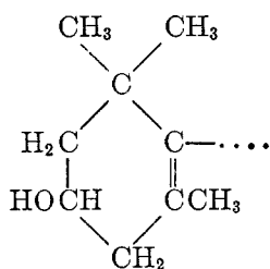
Two terminal groups in zeaxanthin; one such group is present in cryptoxanthin
