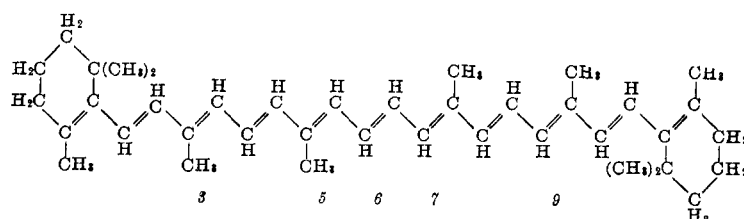
All- trans - \beta -carotene (The five stereochemically effective double bonds are numbered)
