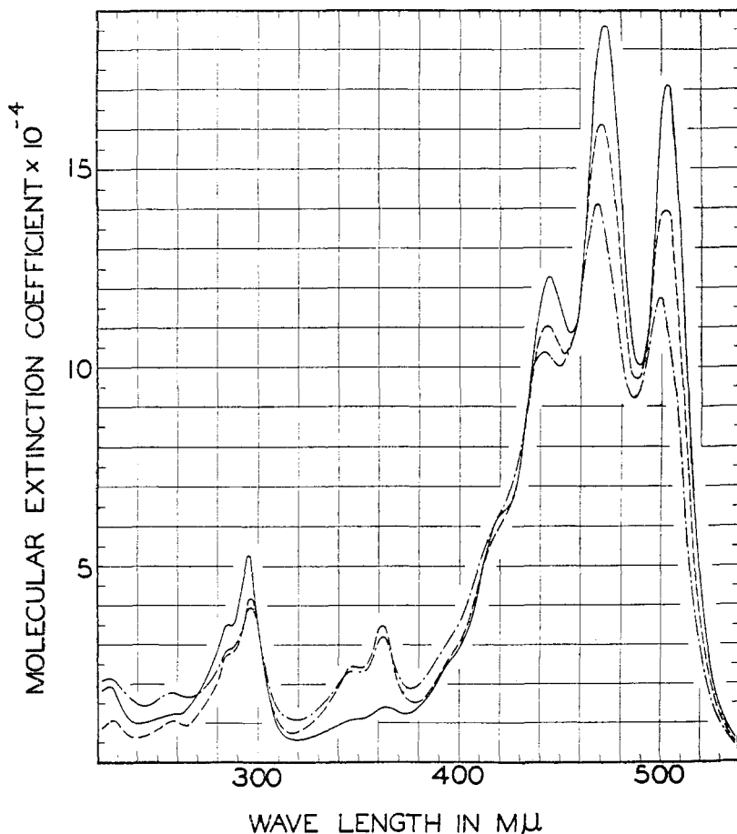
FIG. 9. Molecular extinction curves of lycopene in hexane: —, fresh solution of the all- trans compound; — —, mixture of stereoisomers after refluxing in darkness for 45 min.; — · —, mixture of stereoisomers after iodine catalysis at room temperature in light. (From J. Am. Chem. Soc. 65 , 1942 (1943))
