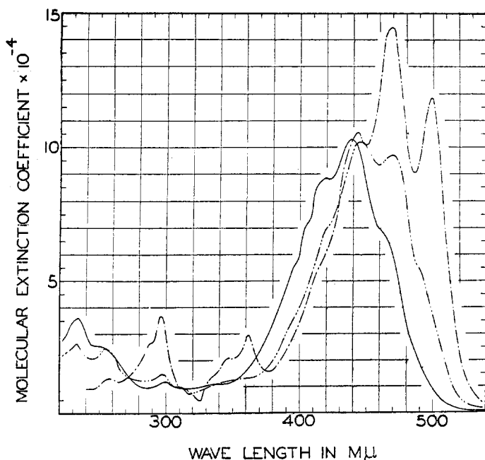
FIG. 16. Molecular extinction curves of polycopene and an unnamed crystalline stereoisomer in hexane: —, fresh solution of polycopene; - - -, fresh solution of the isomer; - · - ·, mixture of stereoisomers in the polycopene solution after iodine catalysis at room temperature in light. (From J. Am. Chem. Soc. 65 , 1943 (1943))
