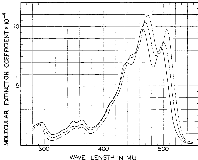
FIG. 33. Molecular extinction curves of neomethylbixin C in benzene: —, fresh solution of neomethylbixin C; ---, mixture of stereoisomers after refluxing in darkness for 45 min.; —·—, mixture of stereoisomers after iodine catalysis at room temperature in light. (From J. Am. Chem. Soc. 66 , 325 (1944))
