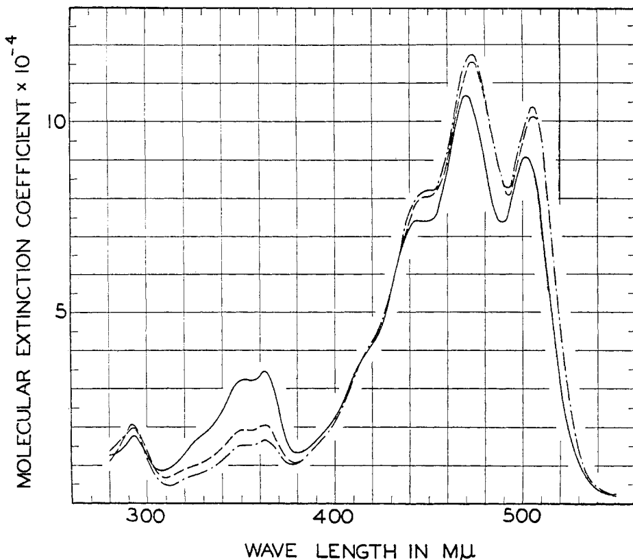
FIG. 32. Molecular extinction curves of neomethylbixin A in benzene: —, fresh solution of neomethylbixin A; ---, mixture of stereoisomers after refluxing in darkness for 45 min.; —·—, mixture of stereoisomers after iodine catalysis at room temperature in light. (From J. Am. Chem. Soc. 66 , 324 (1944))
