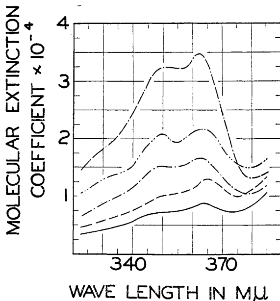
FIG. 37. Molecular extinction curves of some members of the stereoisomeric methylbixin set in the cis -peak region in benzene: —, all- trans -methylbixin; ---, natural methylbixin; —·—, iodine equilibrium mixture; ····, neomethylbixin C; - - - -, neomethylbixin A. (From J. Am. Chem. Soc. 66 , 327 (1944))
