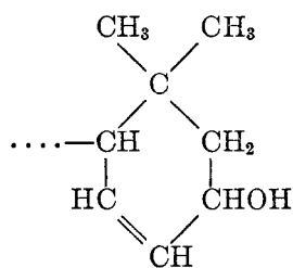
One terminal group in lutein; the other is identical with the formula at the left
